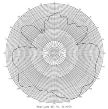
5950 MHz – Azimuth
