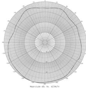
2700 MHz – Azimuth
