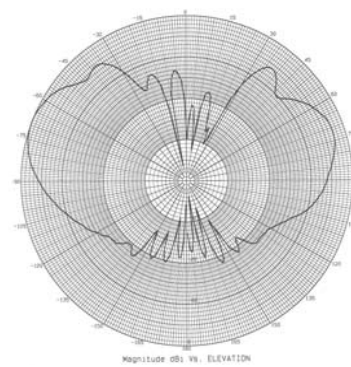
5500 MHz – Elevation
