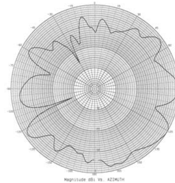
5500 MHz – Azimuth
