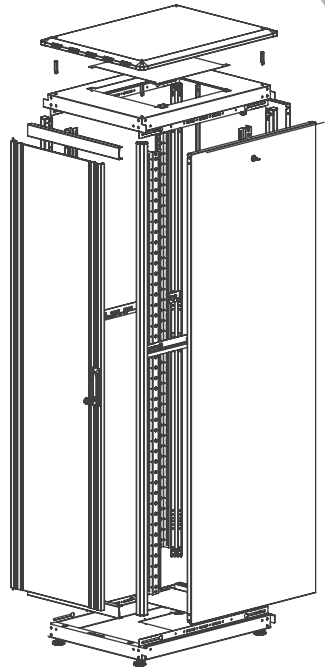
EXPLODED VIEW
